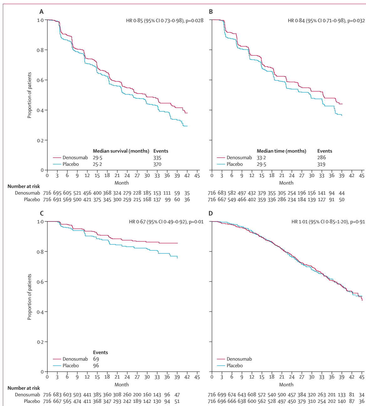
Figure 2: Kaplan-Meier curves of key efficacy endpoints
